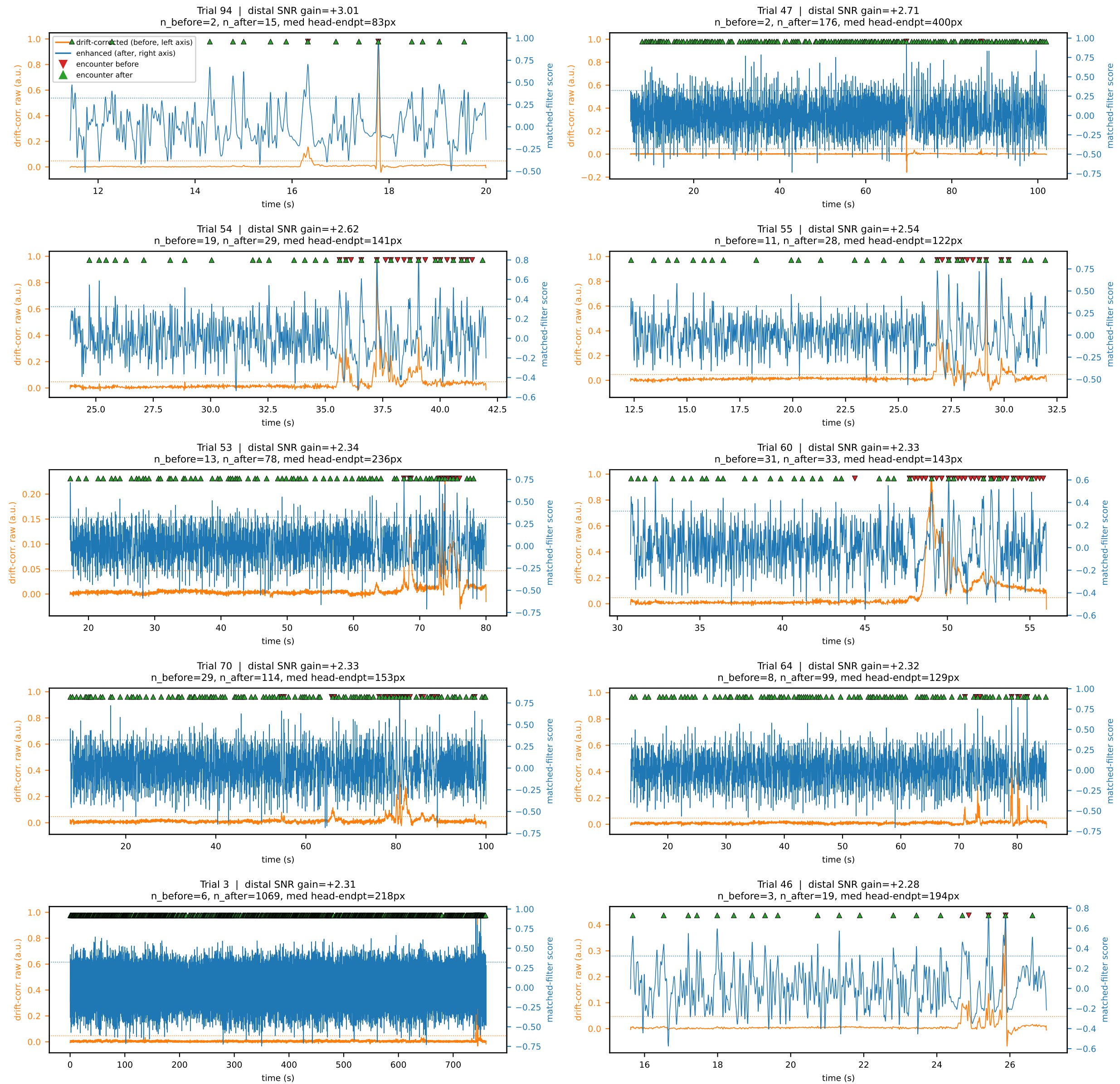
Figure A - Top-10 most distal-SNR-improved ethanol trials: drift-corrected (before) vs enhanced matched-filter (after), twin y-axes, with detected encounters
